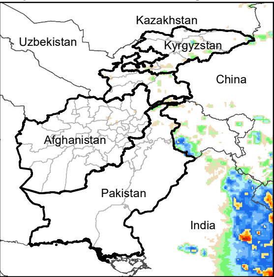
Daily Rainfall estimate for 30 Aug., 2013
