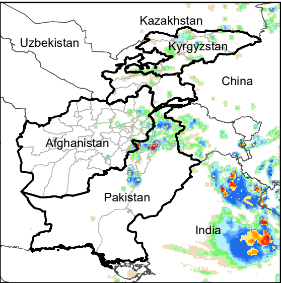
Daily Rainfall estimate for 2 Sep., 2013
