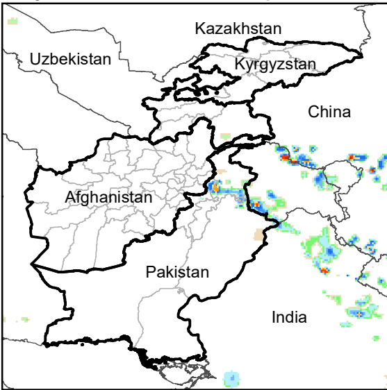
Daily Rainfall estimate for 11 Sep., 2013
