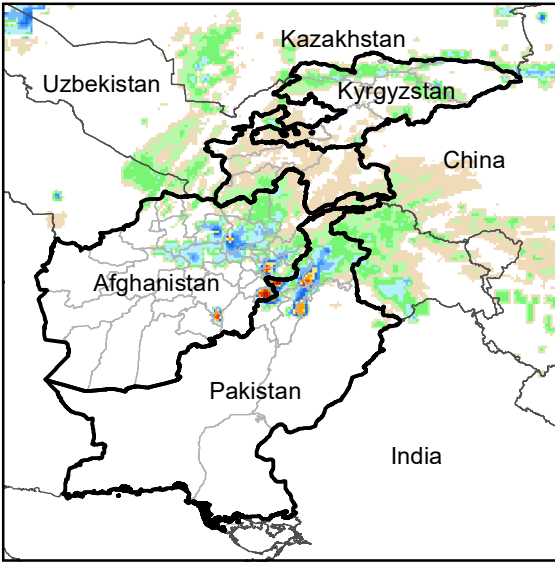
Daily Rainfall estimate for 30 Oct., 2013
