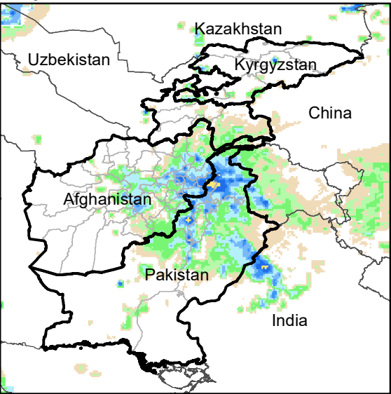
Daily Rainfall estimate for 9 Nov., 2013
