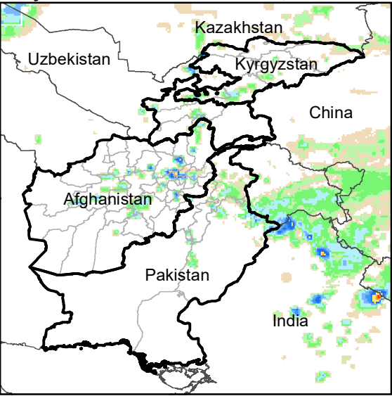
Daily Rainfall estimate for 8 Nov., 2013
