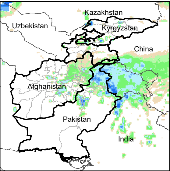
Daily Rainfall estimate for 10 Nov., 2013
