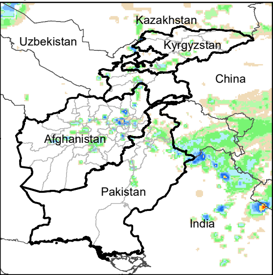
Daily Rainfall estimate for 11 Nov., 2013
