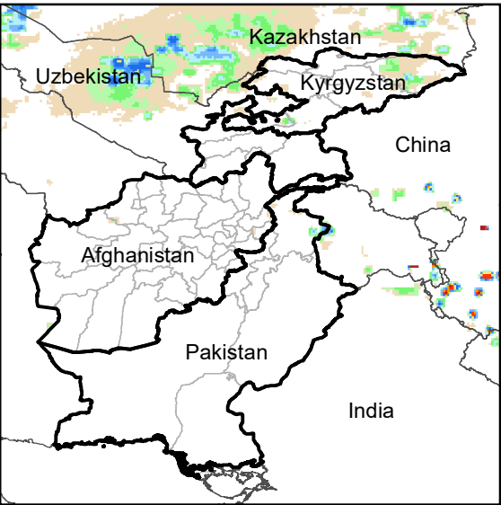
Daily Rainfall estimate for 2 Dec., 2013
