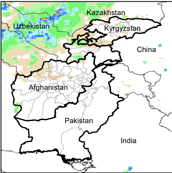
Daily Rainfall estimate for 7 Dec., 2013
