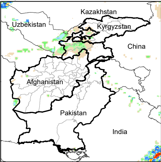
Daily Rainfall estimate for 26 Feb., 2014
