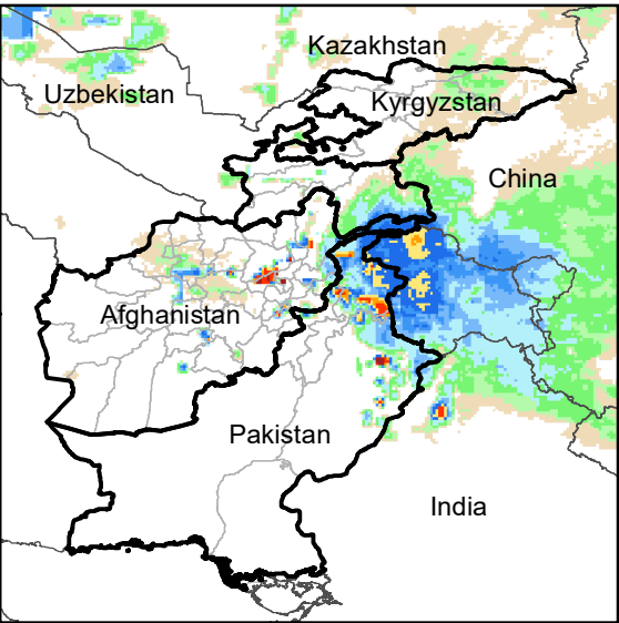
Daily Rainfall estimate for 21 Mar., 2014
