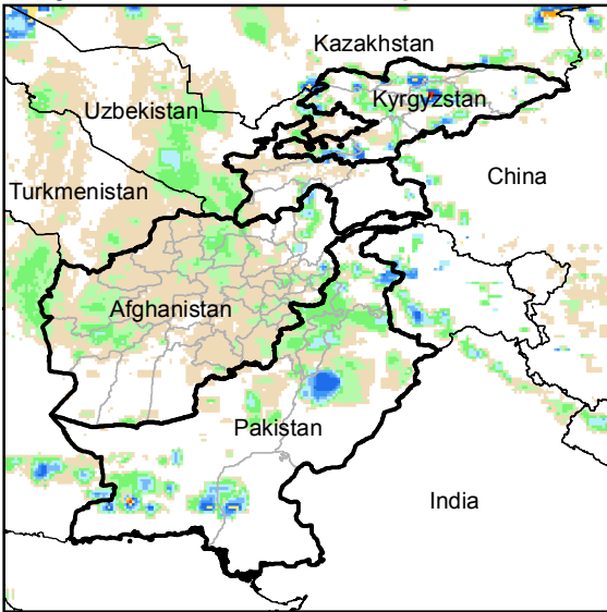
Daily Rainfall estimate for 4 Apr., 2014
