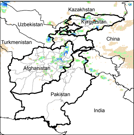
Daily Rainfall estimate for 2 Apr., 2014
