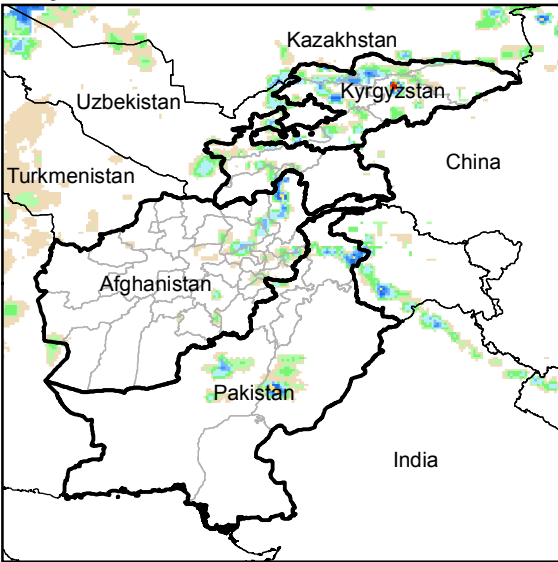
Daily Rainfall estimate for 3 Apr., 2014
