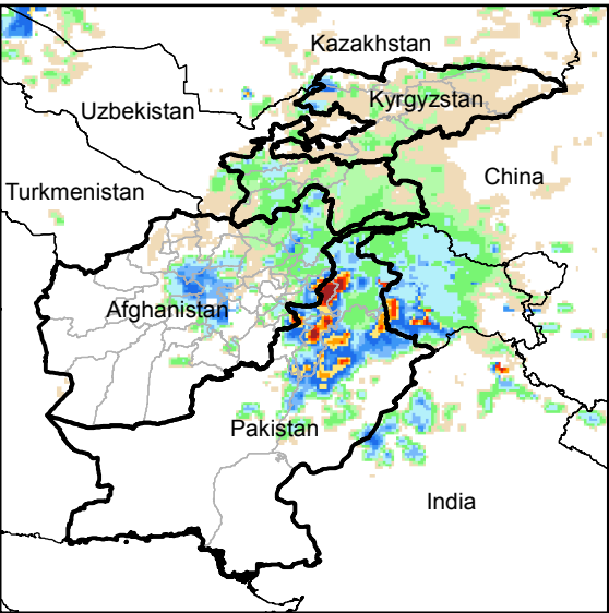
Daily Rainfall estimate for 9 Apr., 2014
