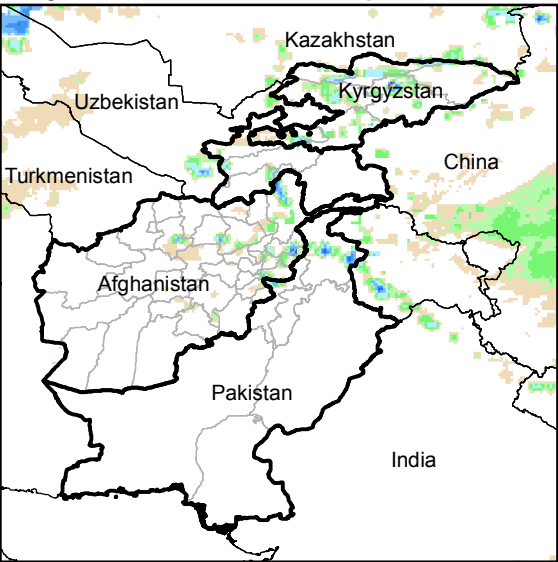
Daily Rainfall estimate for 12 Apr., 2014
