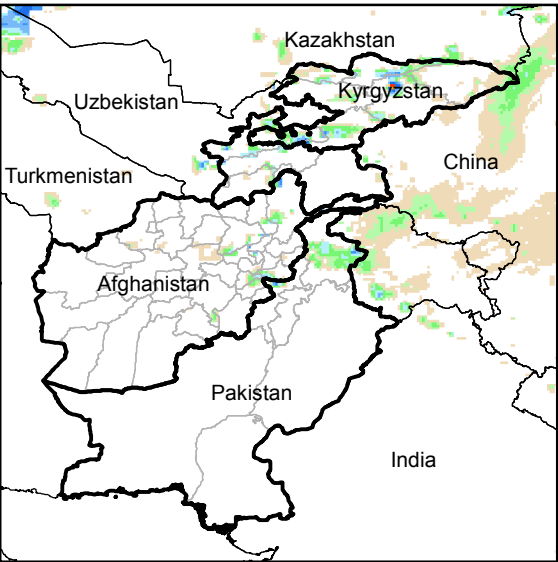
Daily Rainfall estimate for 11 Apr., 2014
