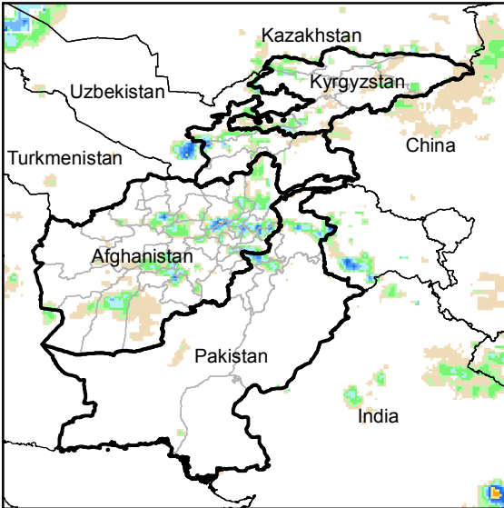
Daily Rainfall estimate for 14 Apr., 2014
