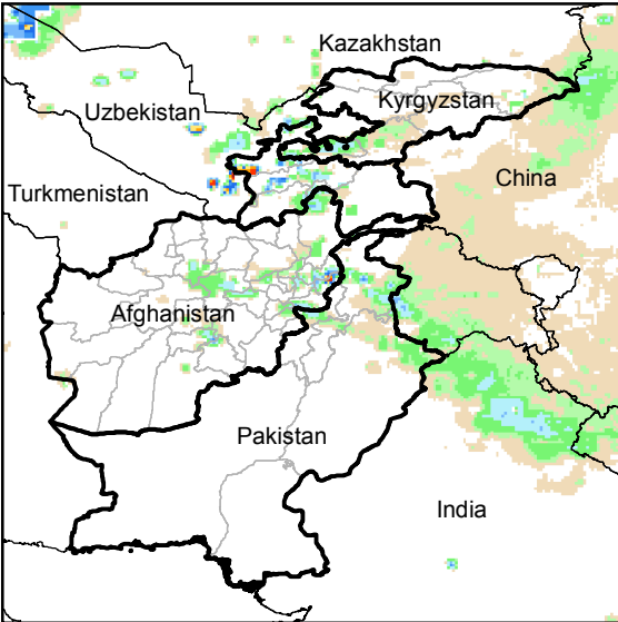
Daily Rainfall estimate for 13 Apr., 2014
