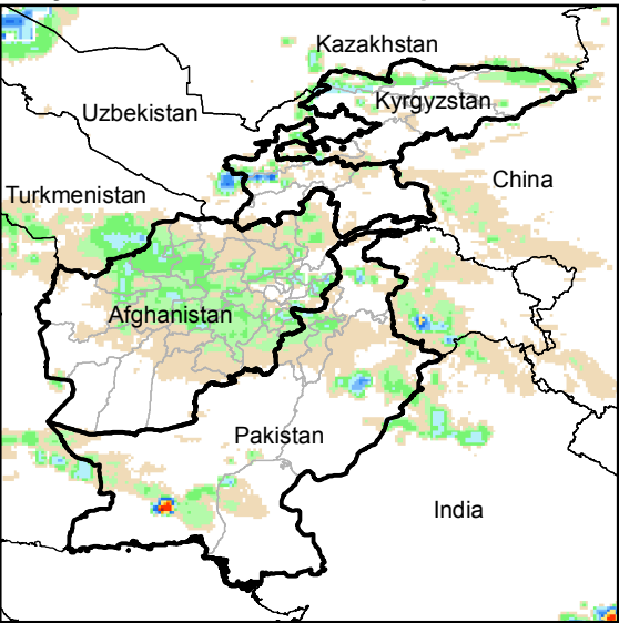
Daily Rainfall estimate for 18 Apr., 2014
