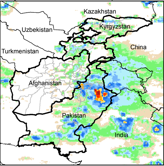
Daily Rainfall estimate for 17 Apr., 2014
