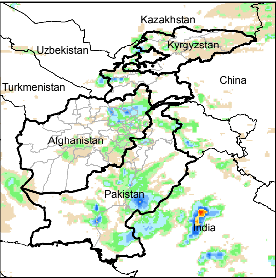
Daily Rainfall estimate for 25 Apr., 2014
