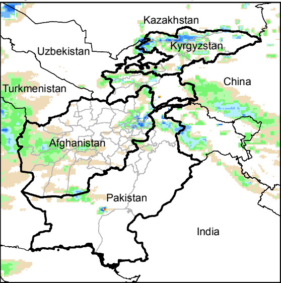
Daily Rainfall estimate for 26 Apr., 2014
