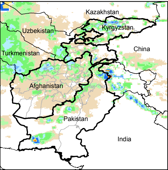
Daily Rainfall estimate for 27 Apr., 2014
