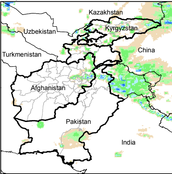
Daily Rainfall estimate for 29 Apr., 2014
