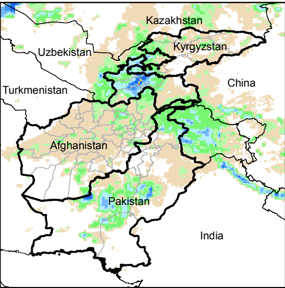
Daily Rainfall estimate for 28 Apr., 2014
