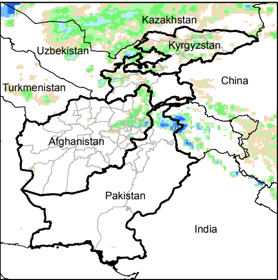
Daily Rainfall estimate for 30 Apr., 2014
