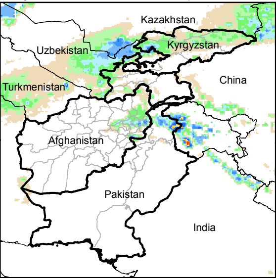
Daily Rainfall estimate for 1 May., 2014
