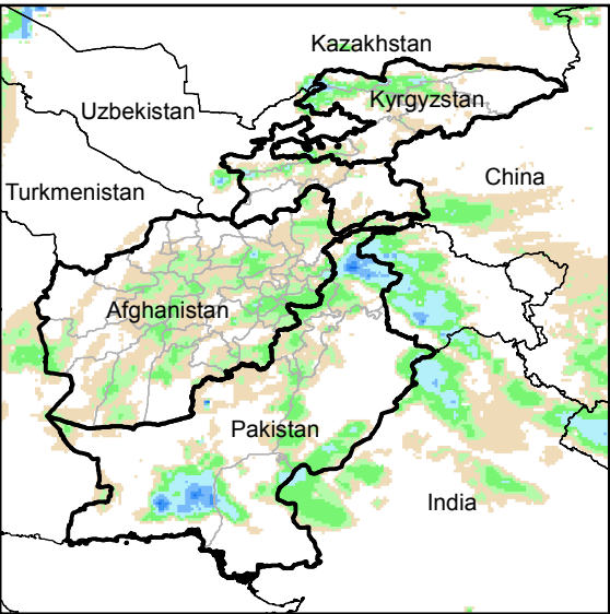
Daily Rainfall estimate for 5 May., 2014
