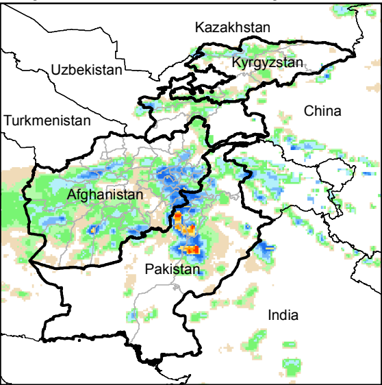
Daily Rainfall estimate for 19 May., 2014
