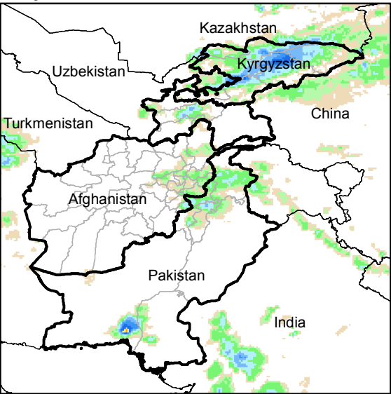
Daily Rainfall estimate for 5 Jun., 2014
