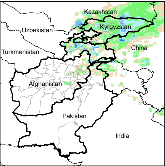
Daily Rainfall estimate for 10 Jun., 2014
