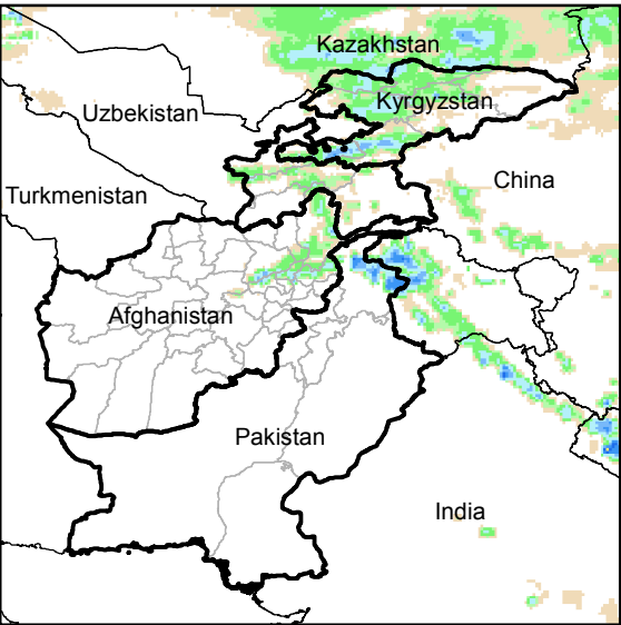
Daily Rainfall estimate for 12 Jun., 2014
