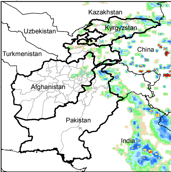
Daily Rainfall estimate for 21 Jun., 2014
