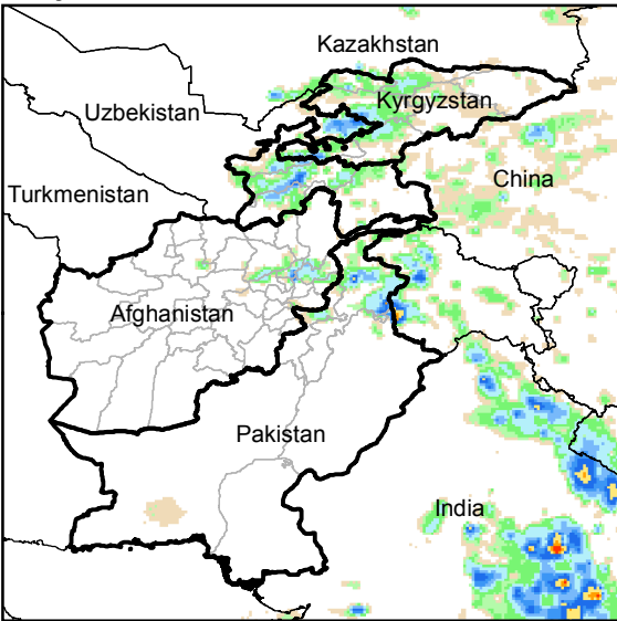
Daily Rainfall estimate for 20 Jun., 2014
