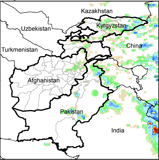
Daily Rainfall estimate for 22 Jun., 2014
