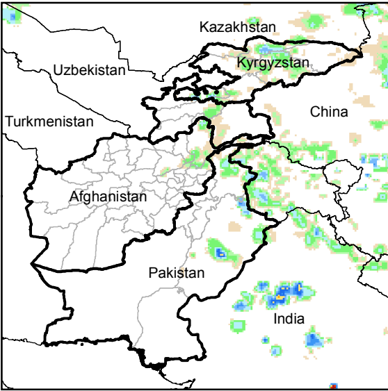
Daily Rainfall estimate for 24 Jun., 2014
