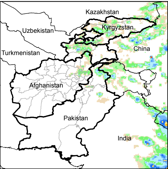
Daily Rainfall estimate for 23 Jun., 2014
