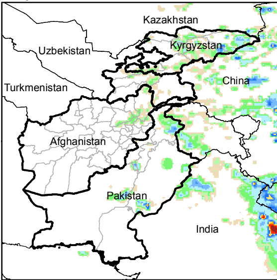
Daily Rainfall estimate for 25 Jun., 2014
