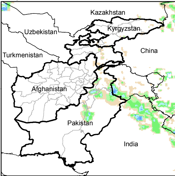
Daily Rainfall estimate for 3 Jul., 2014
