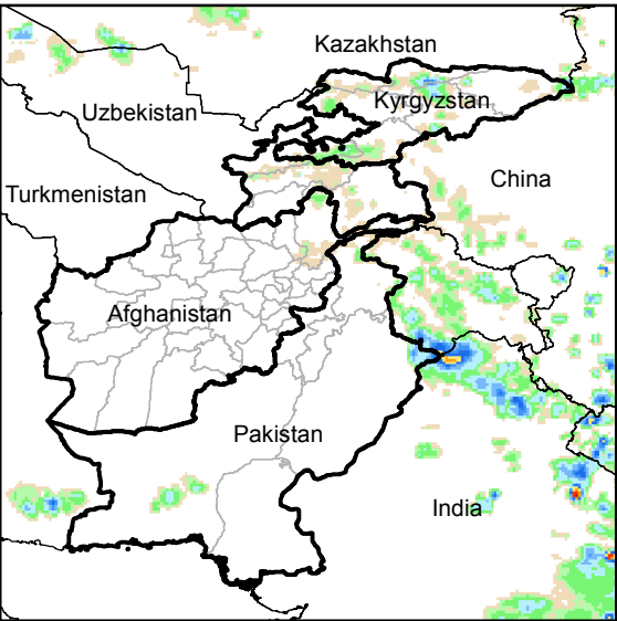
Daily Rainfall estimate for 1 Jul., 2014
