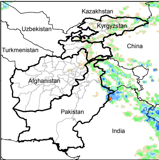
Daily Rainfall estimate for 2 Jul., 2014
