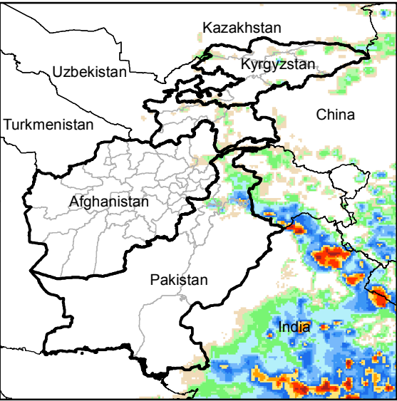
Daily Rainfall estimate for 15 Jul., 2014
