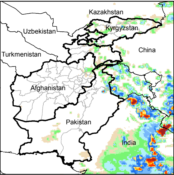
Daily Rainfall estimate for 14 Jul., 2014
