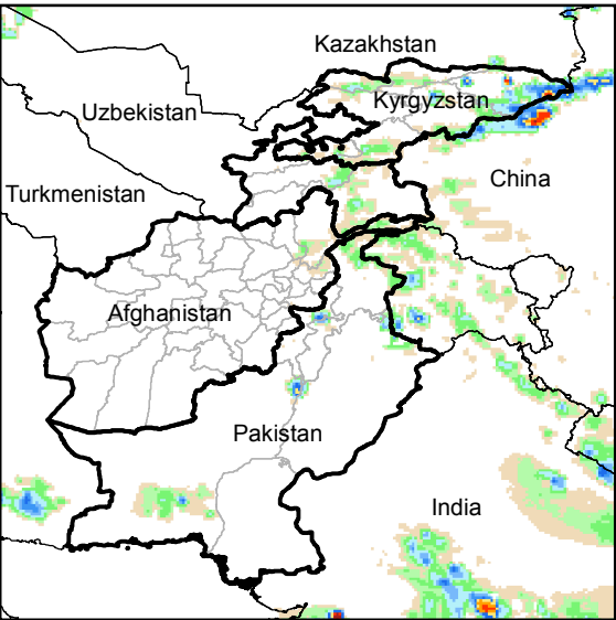
Daily Rainfall estimate for 13 Jul., 2014
