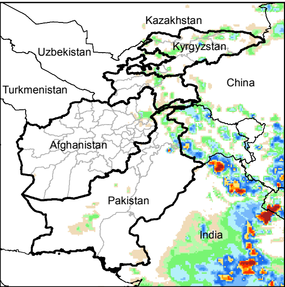
Daily Rainfall estimate for 17 Jul., 2014
