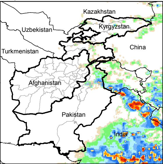
Daily Rainfall estimate for 18 Jul., 2014
