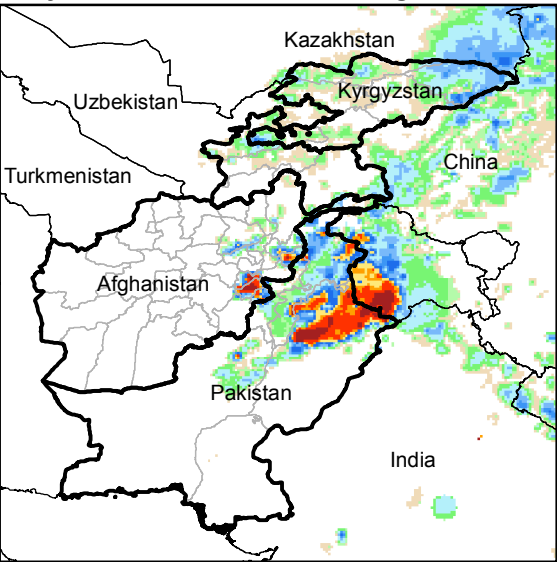
Daily Rainfall estimate for 19 Aug., 2014
