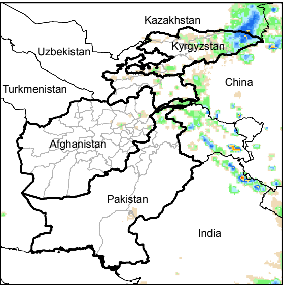
Daily Rainfall estimate for 21 Aug., 2014
