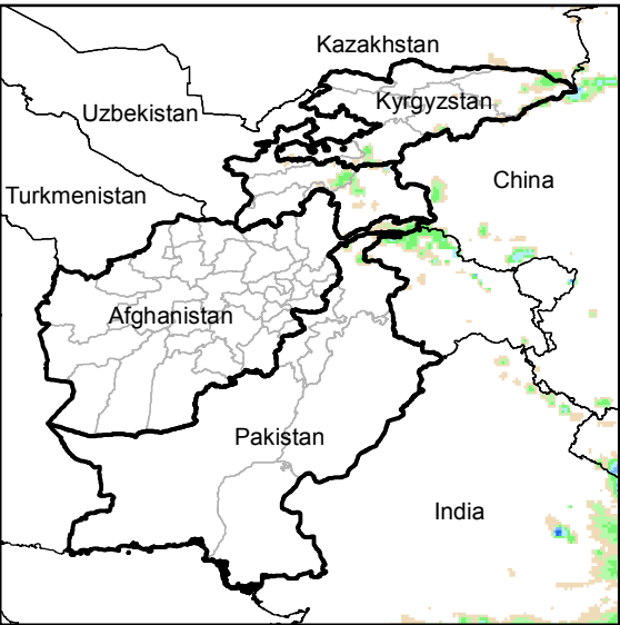
Daily Rainfall estimate for 23 Aug., 2014
