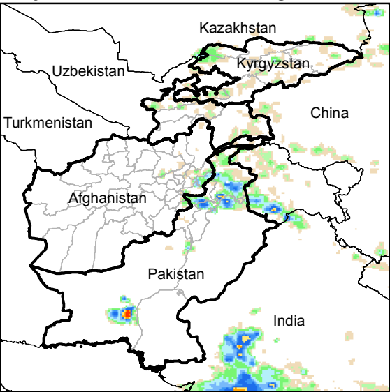
Daily Rainfall estimate for 28 Aug., 2014
