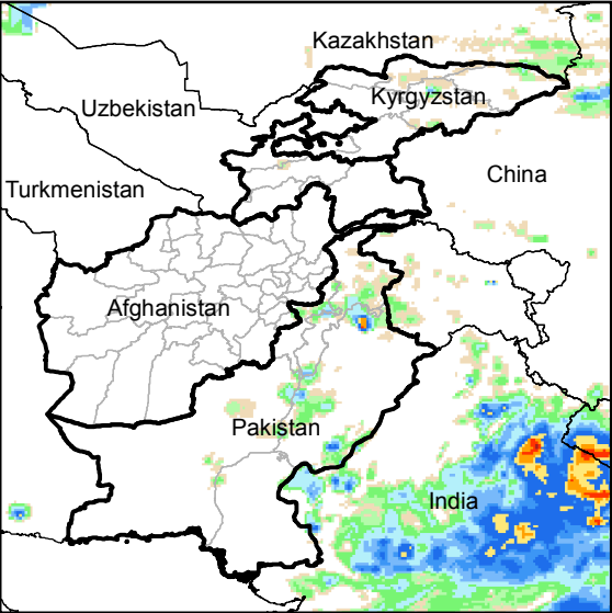
Daily Rainfall estimate for 11 Sep., 2014
