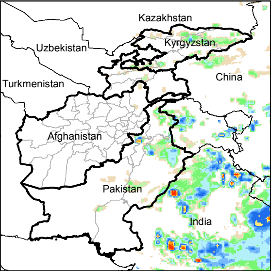
Daily Rainfall estimate for 12 Sep., 2014
