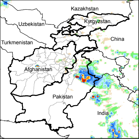
Daily Rainfall estimate for 14 Sep., 2014
