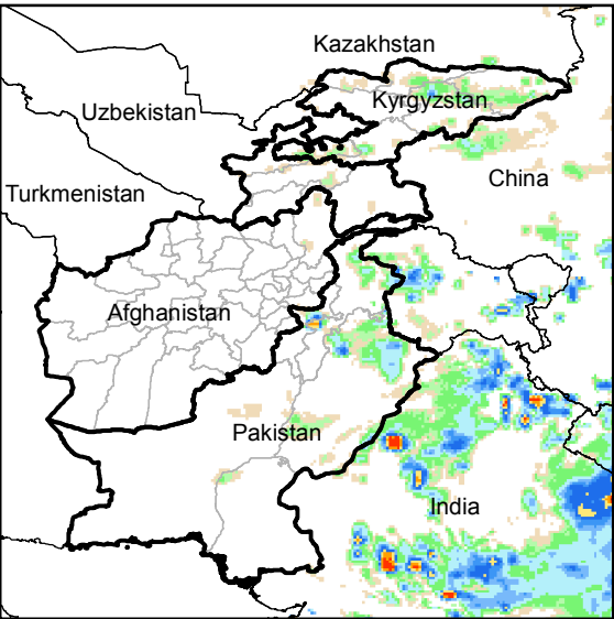
Daily Rainfall estimate for 15 Sep., 2014
