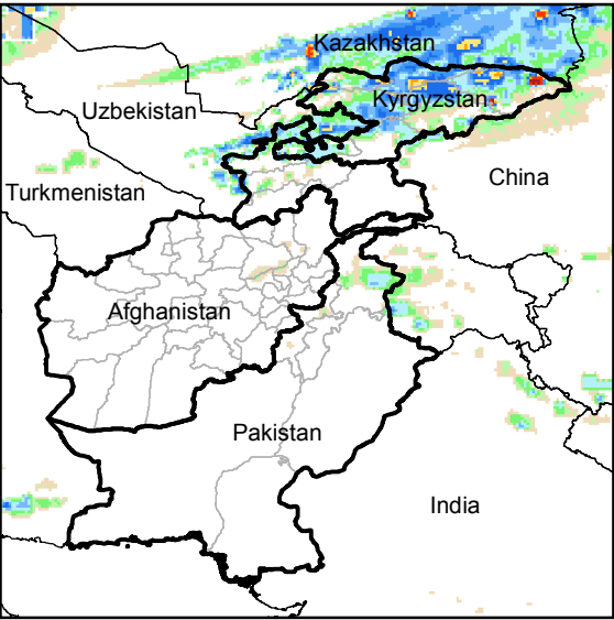
Daily Rainfall estimate for 4 Oct., 2014
