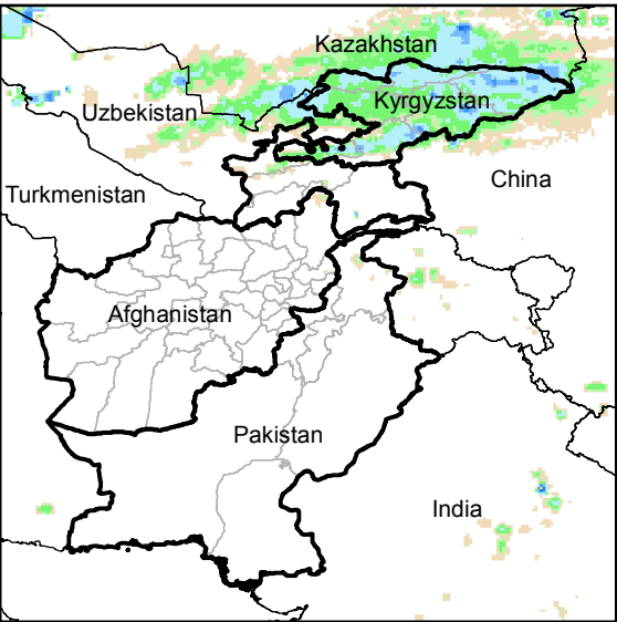
Daily Rainfall estimate for 5 Oct., 2014
