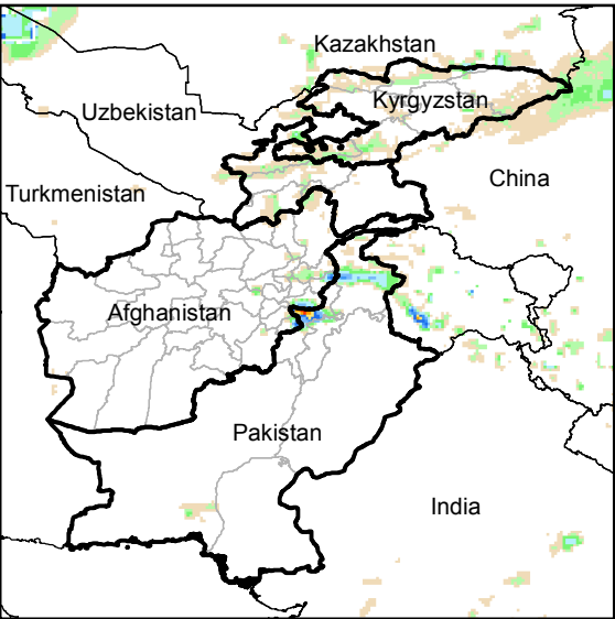
Daily Rainfall estimate for 12 Oct., 2014
