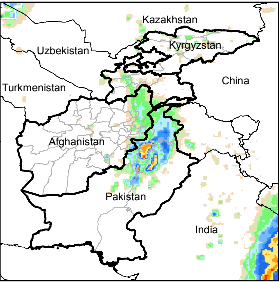
Daily Rainfall estimate for 13 Oct., 2014
