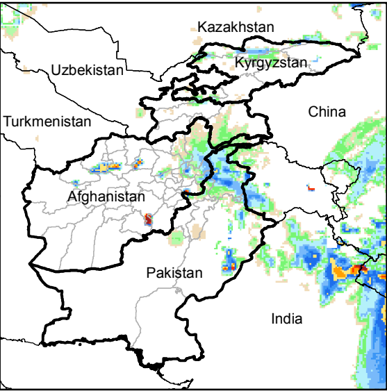
Daily Rainfall estimate for 14 Oct., 2014
