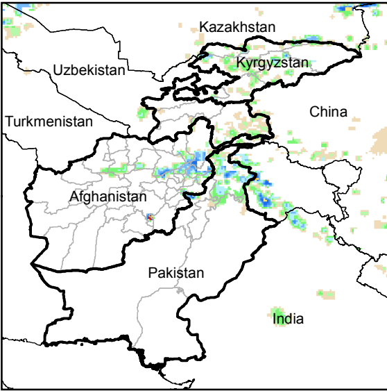
Daily Rainfall estimate for 15 Oct., 2014
