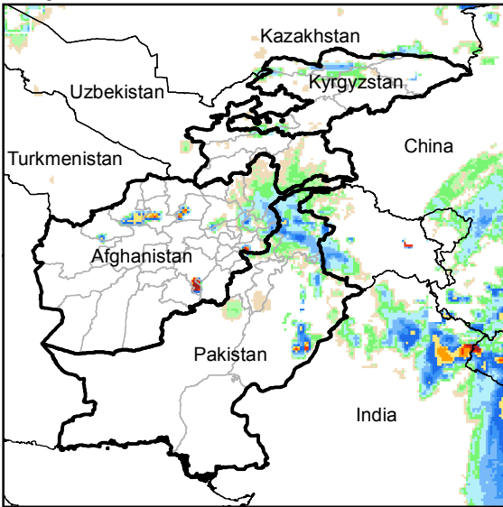
Daily Rainfall estimate for 17 Oct., 2014
