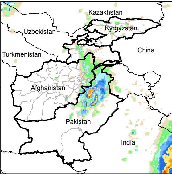
Daily Rainfall estimate for 16 Oct., 2014
