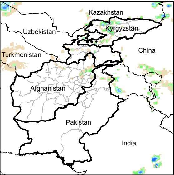
Daily Rainfall estimate for 20 Oct., 2014
