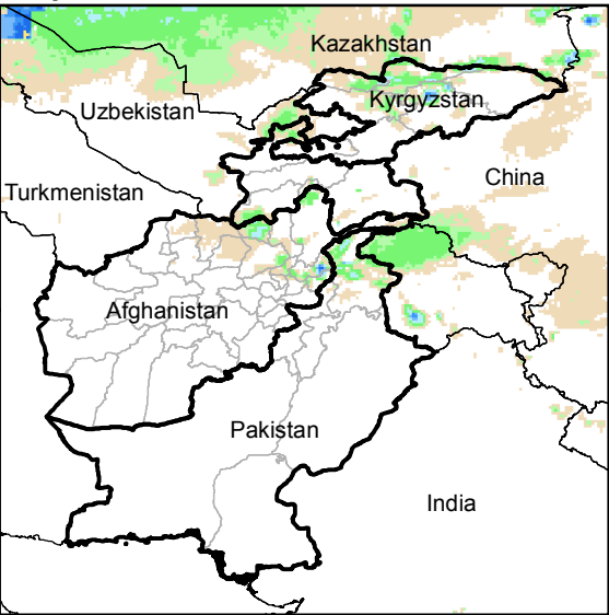
Daily Rainfall estimate for 23 Oct., 2014
