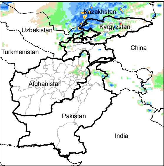
Daily Rainfall estimate for 24 Oct., 2014
