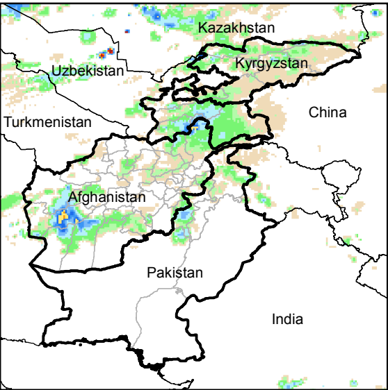
Daily Rainfall estimate for 22 Oct., 2014
