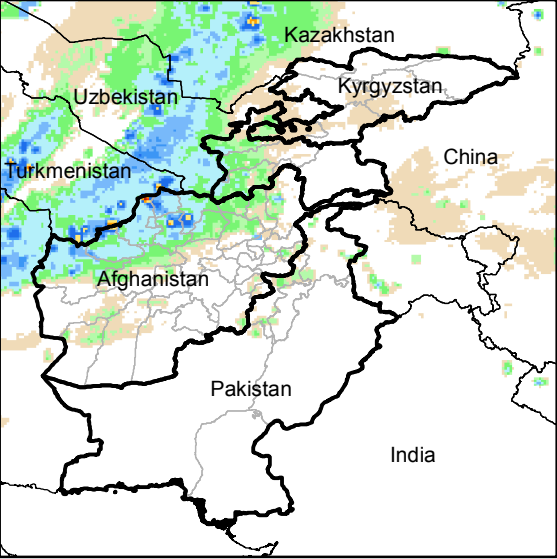
Daily Rainfall estimate for 5 Nov., 2014
