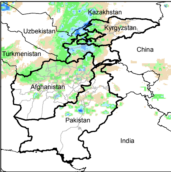
Daily Rainfall estimate for 6 Nov., 2014
