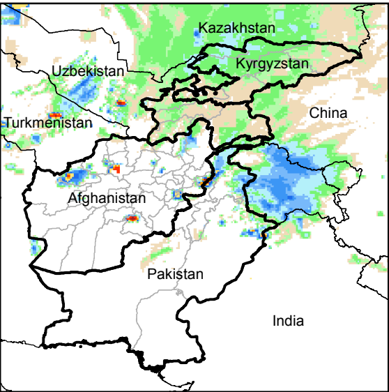
Daily Rainfall estimate for 10 Nov., 2014
