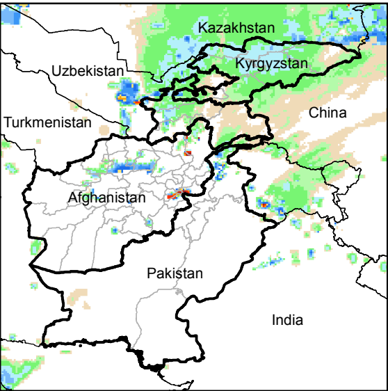
Daily Rainfall estimate for 11 Nov., 2014
