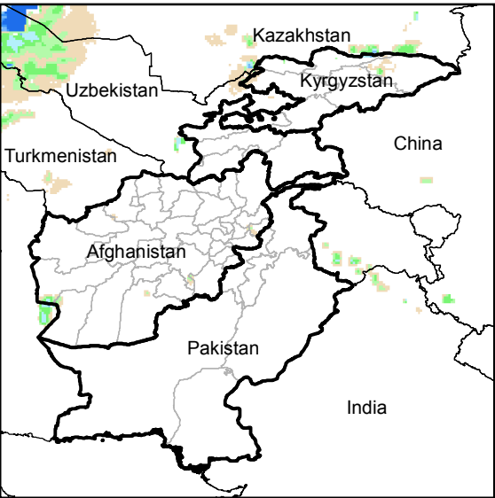
Daily Rainfall estimate for 26 Nov., 2014
