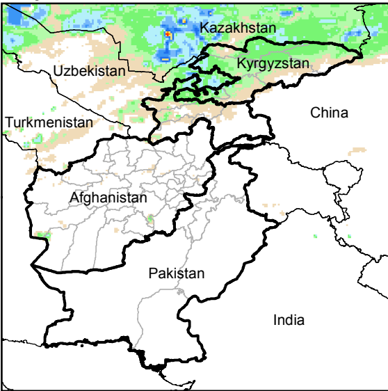
Daily Rainfall estimate for 27 Nov., 2014
