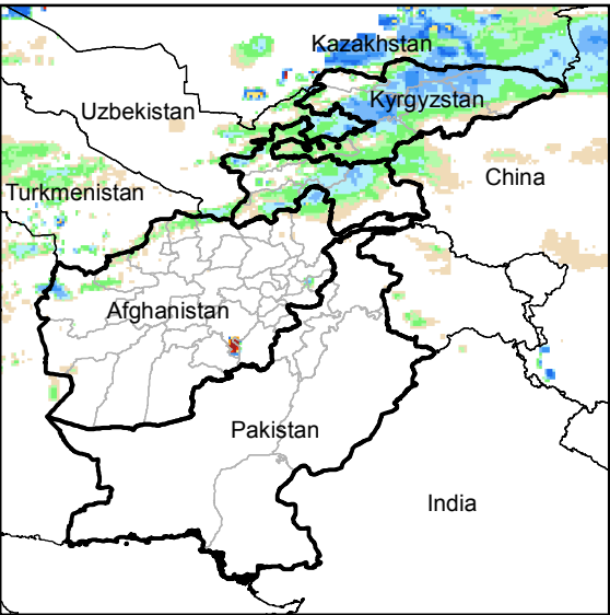
Daily Rainfall estimate for 28 Nov., 2014
