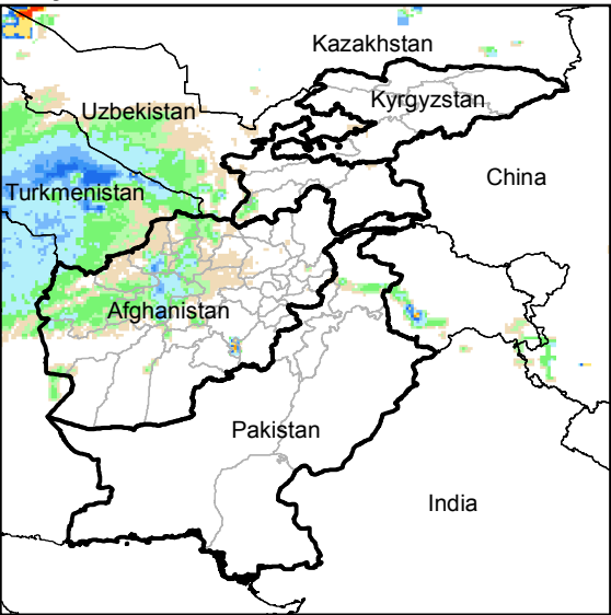
Daily Rainfall estimate for 29 Nov., 2014
